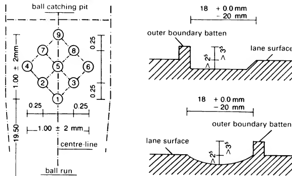
③ Arrangement and numbering of skittles
